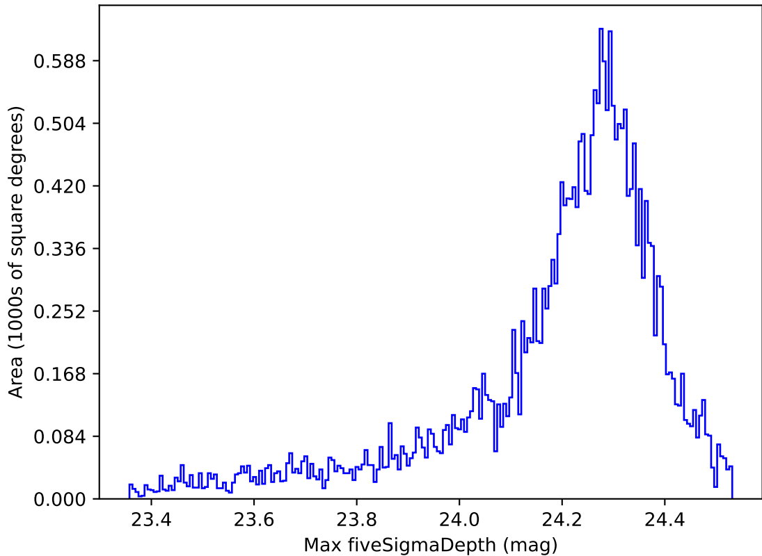
weather_cloudso8v3.4_10yrs All sky i band: Max fiveSigmaDepth
