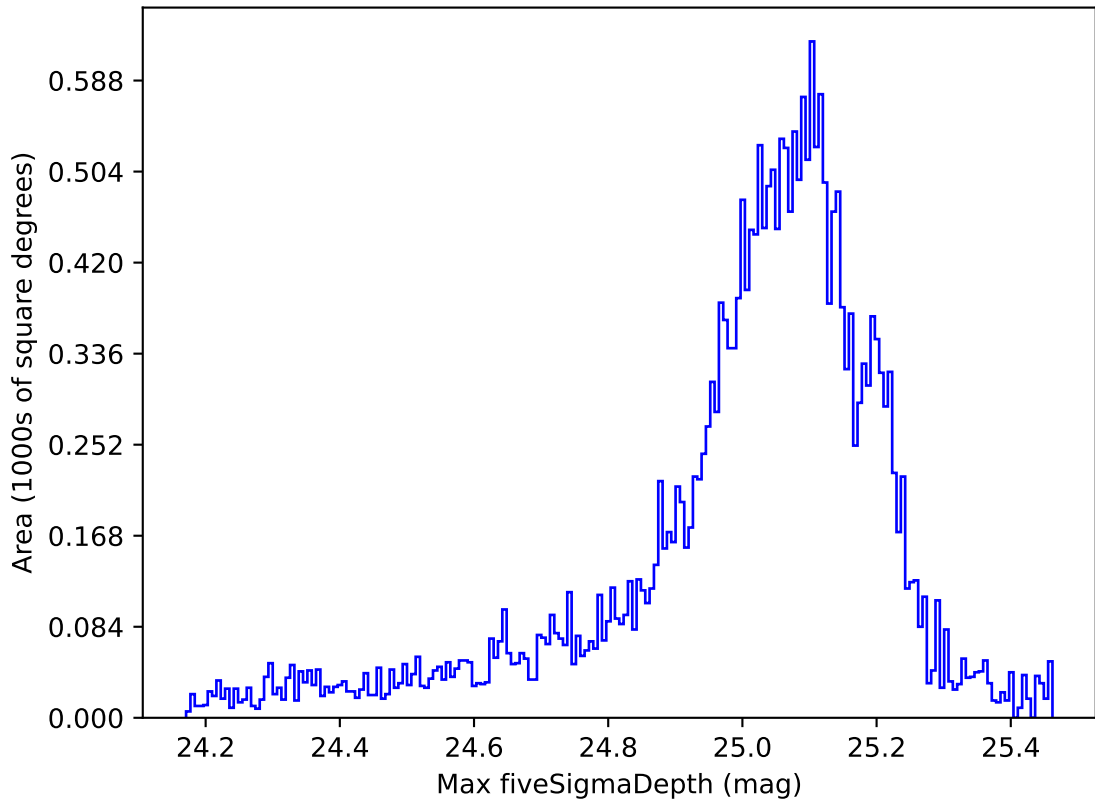
weather_cloudso8v3.4_10yrs All sky g band: Max fiveSigmaDepth
