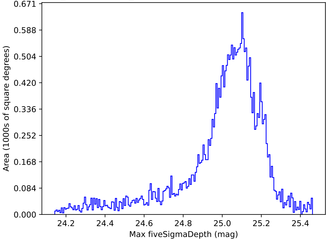
weather_cloudso8v3.4_10yrs All sky all bands: Max fiveSigmaDepth
