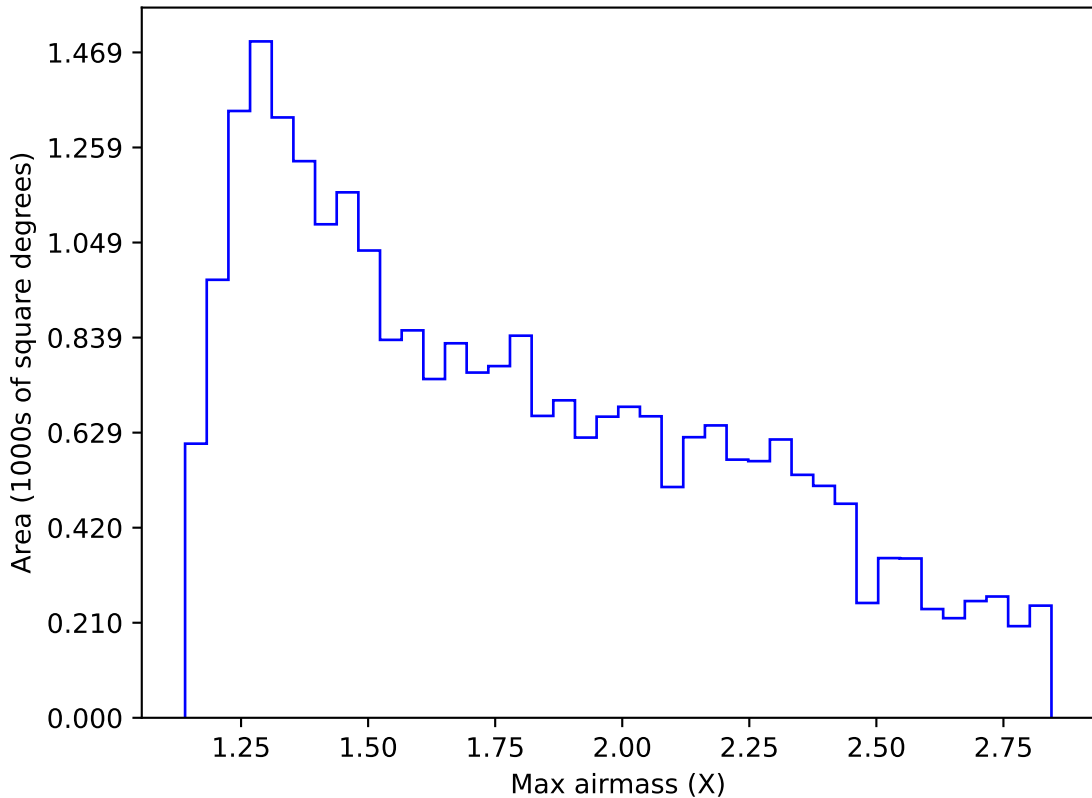
weather_cloudso8v3.4_10yrs Yr 1 z band: Max airmass
