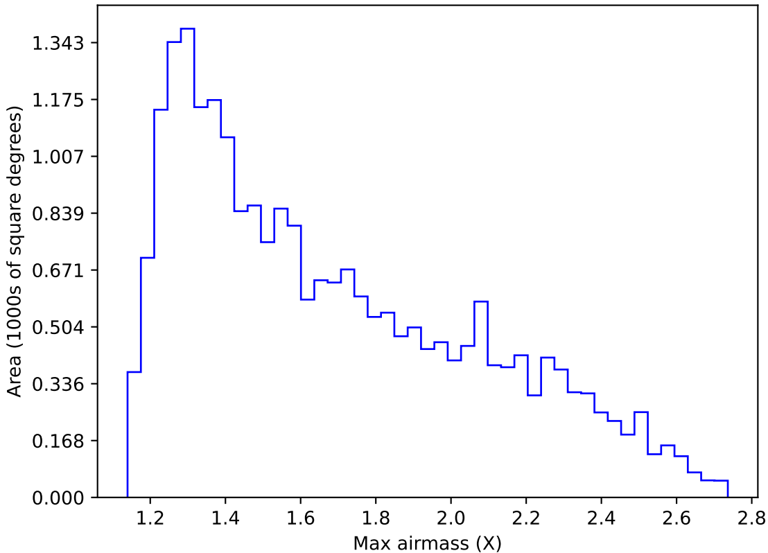
weather_cloudso8v3.4_10yrs Yr 1 y band: Max airmass
