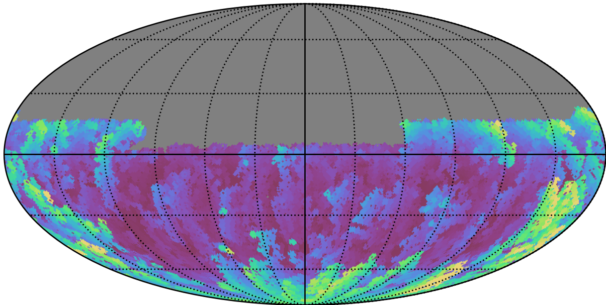
weather_cloudso8v3.4_10yrs Yr 1 u band: Max airmass
