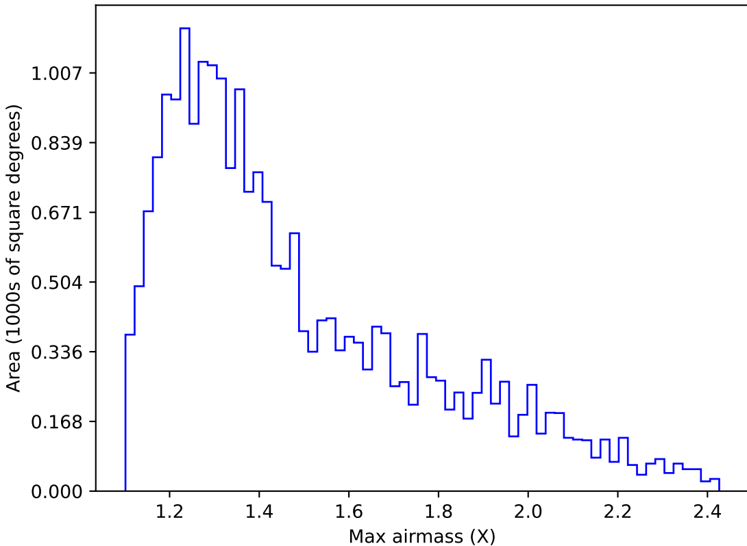
weather_cloudso8v3.4_10yrs Yr 1 u band: Max airmass
