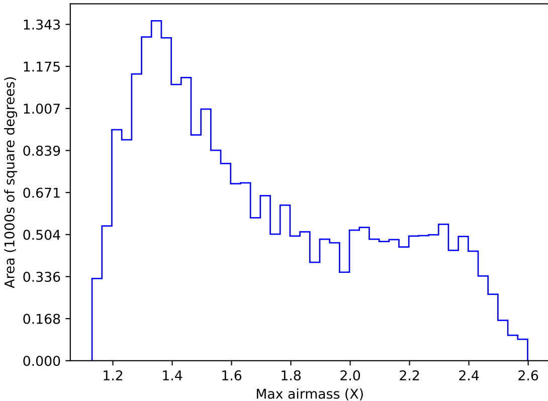
weather_cloudso8v3.4_10yrs Yr 1 r band: Max airmass
