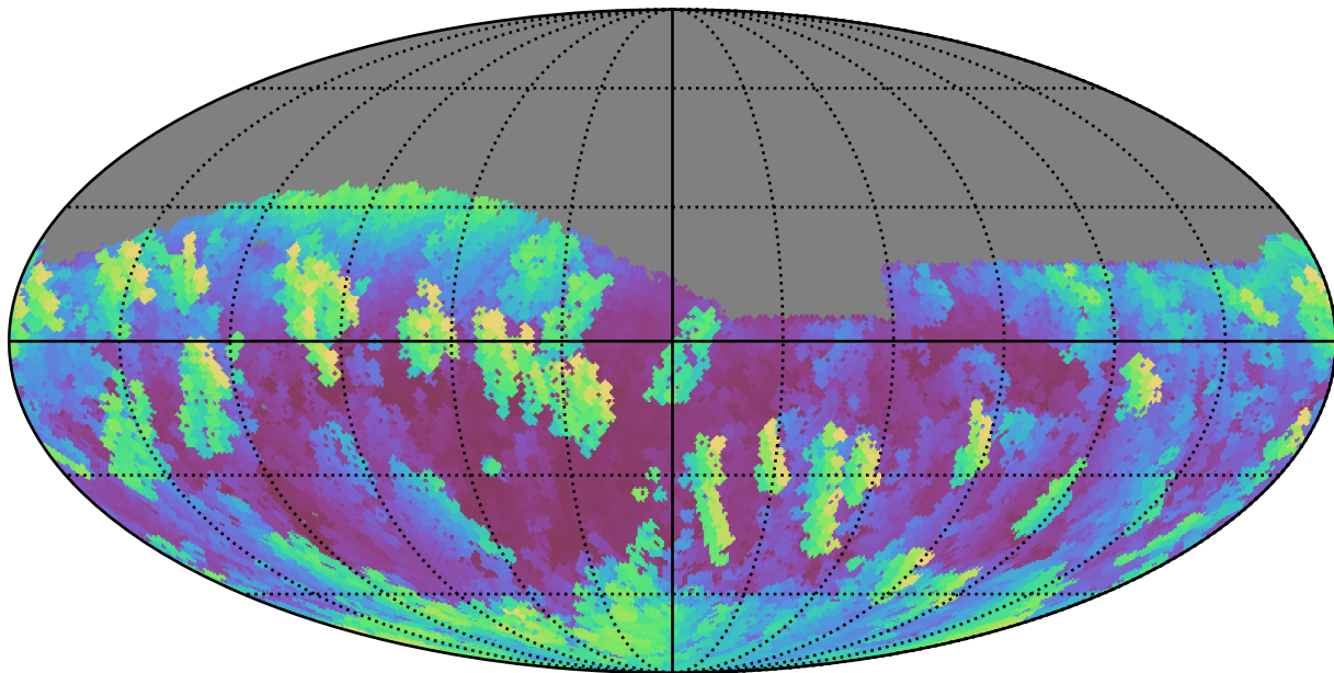
weather_cloudso8v3.4_10yrs Yr 1 i band: Max airmass
