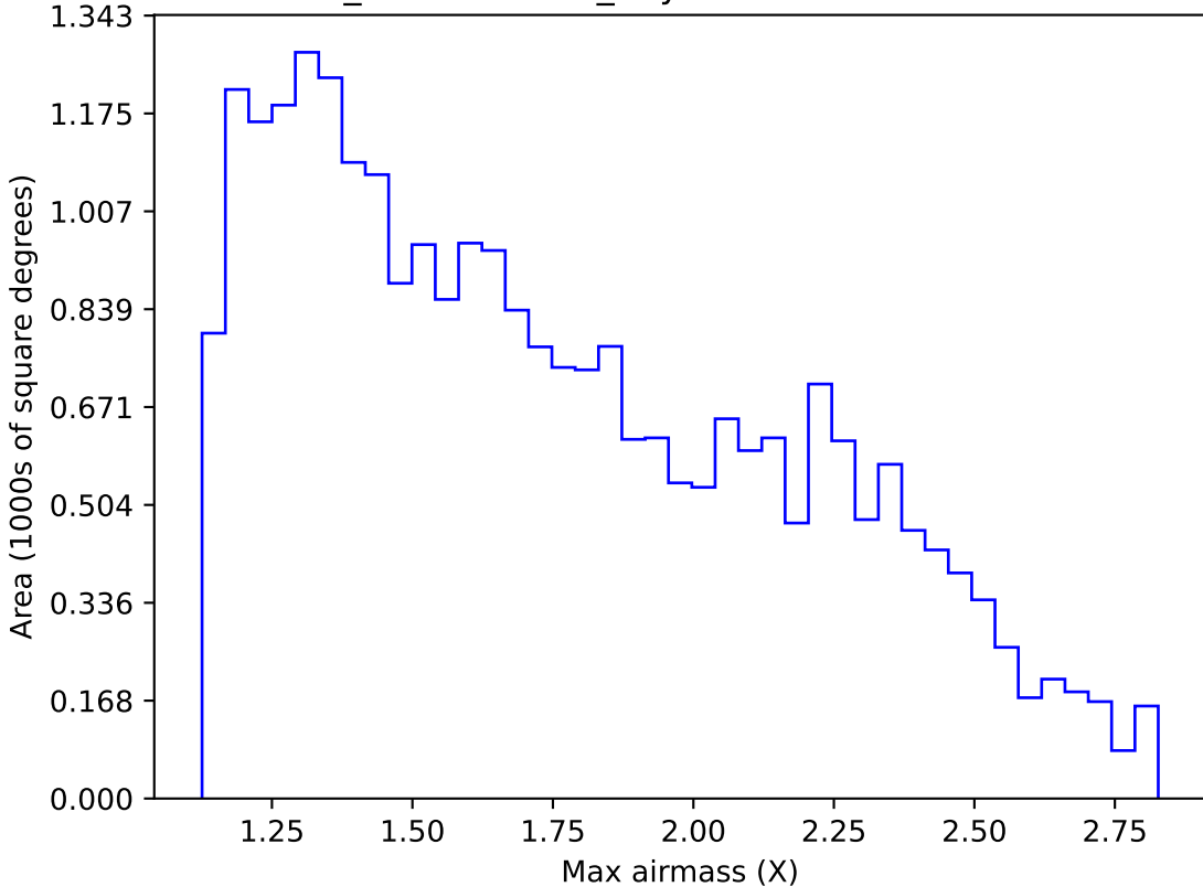
weather_cloudso8v3.4_10yrs Yr 1 i band: Max airmass
