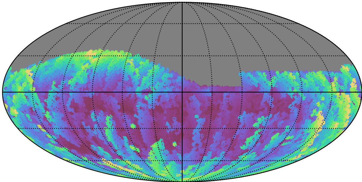
weather_cloudso8v3.4_10yrs Yr 1 g band: Max airmass
