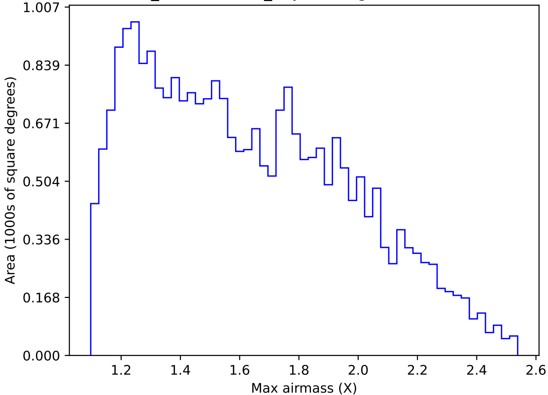
weather_cloudso8v3.4_10yrs Yr 1 g band: Max airmass
