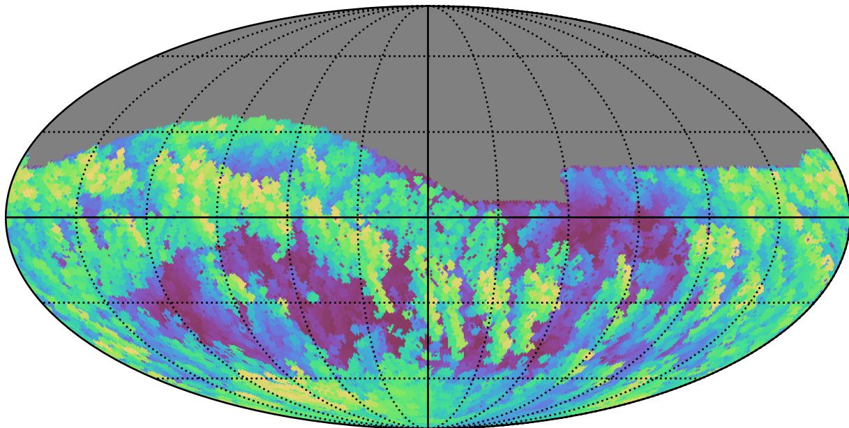
weather_cloudso8v3.4_10yrs Yr 1 all bands: Max airmass
