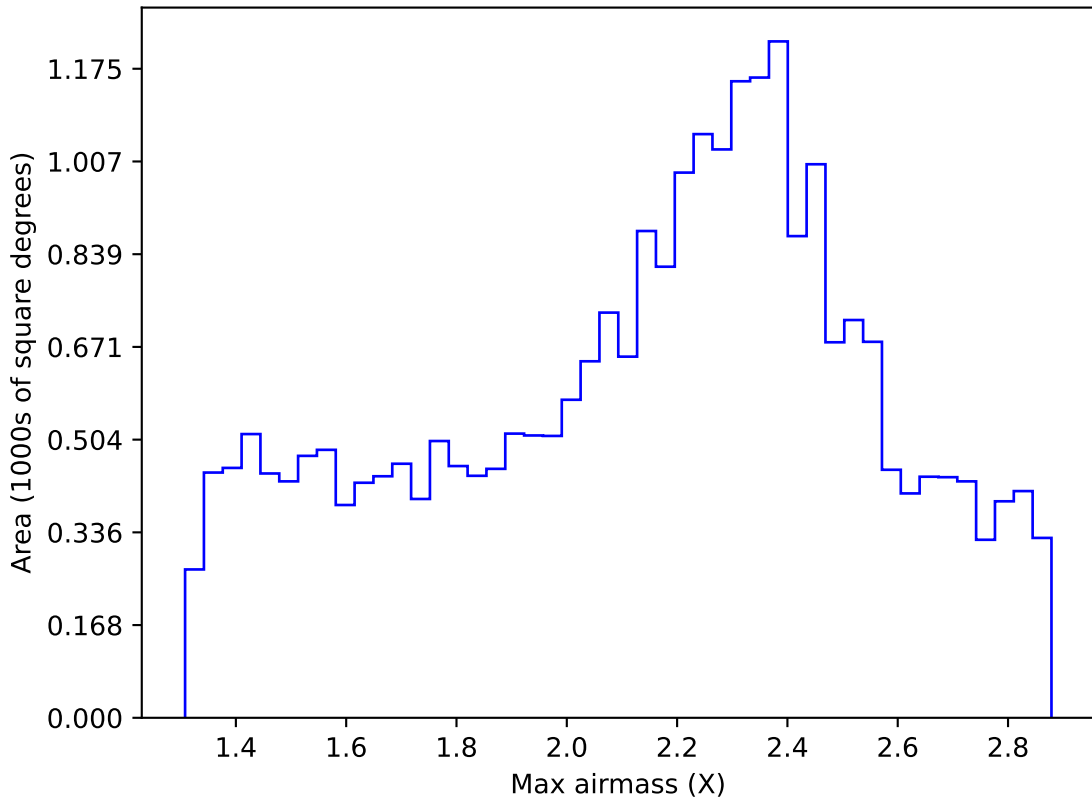
weather_cloudso8v3.4_10yrs Yr 1 all bands: Max airmass
