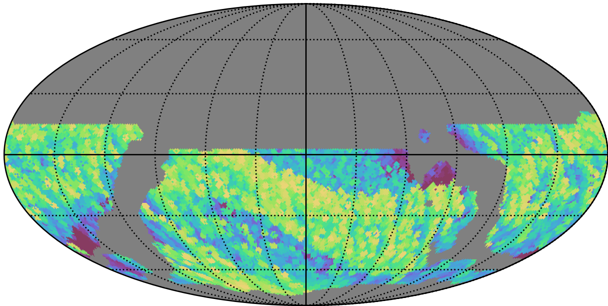
weather_cloudso8v3.4_10yrs WFD z band: Max airmass
