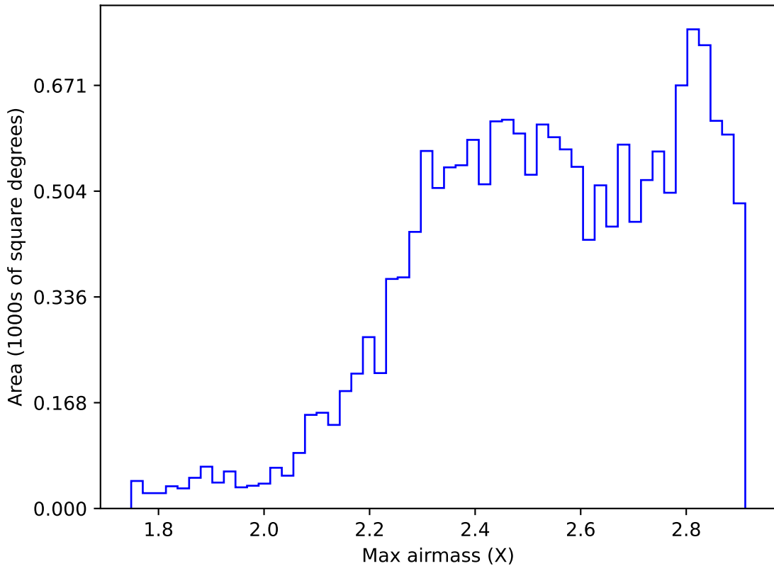
weather_cloudso8v3.4_10yrs WFD z band: Max airmass
