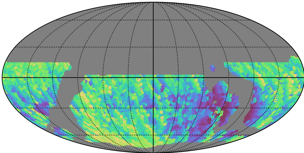
weather_cloudso8v3.4_10yrs WFD y band: Max airmass
