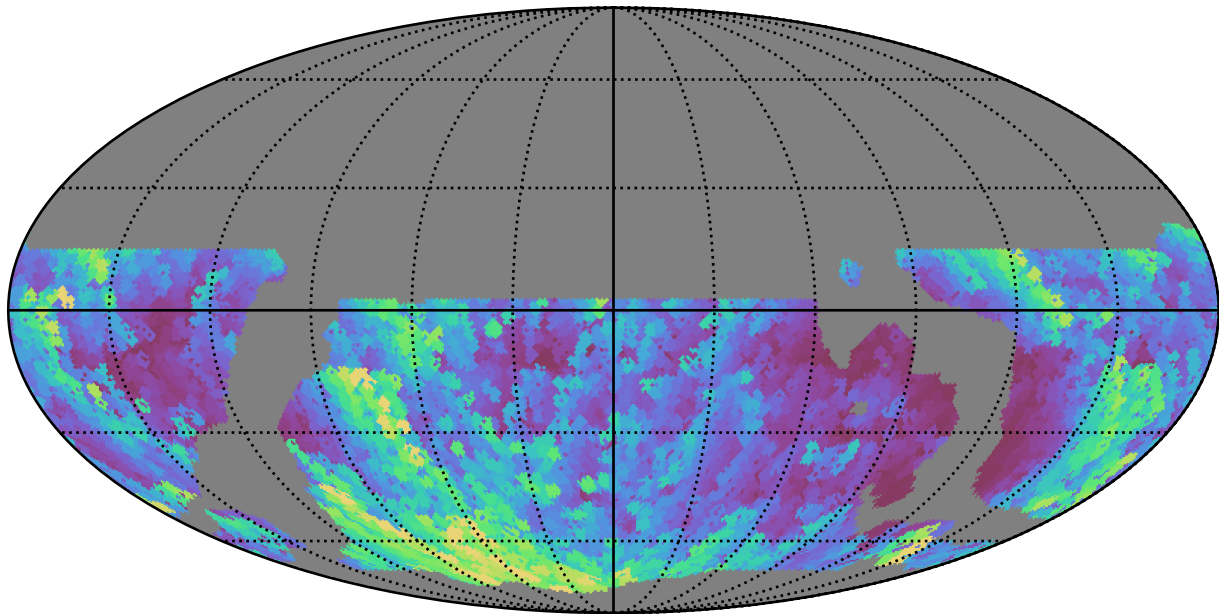
weather_cloudso8v3.4_10yrs WFD u band: Max airmass
