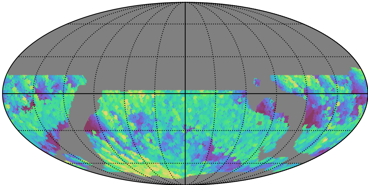
weather_cloudso8v3.4_10yrs WFD r band: Max airmass
