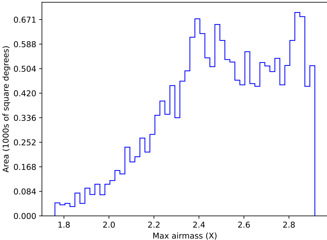
weather_cloudso8v3.4_10yrs WFD i band: Max airmass
