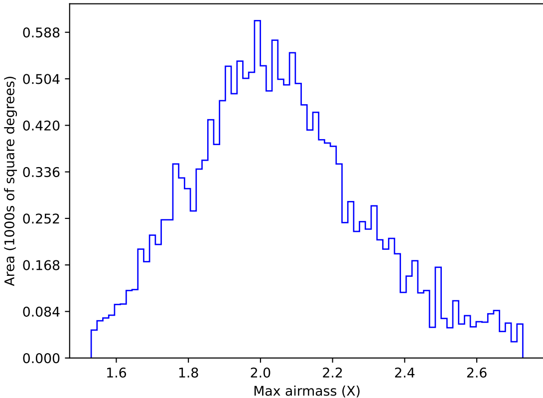
weather_cloudso8v3.4_10yrs WFD g band: Max airmass
