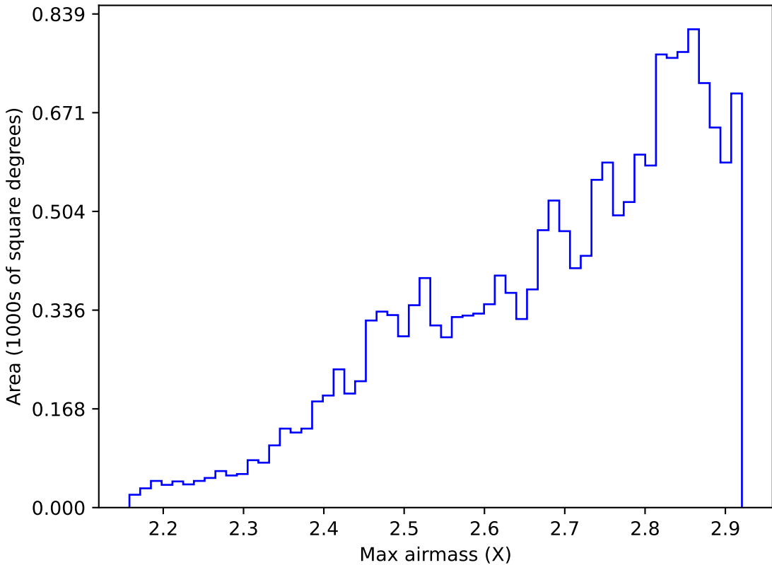
weather_cloudso8v3.4_10yrs WFD all bands: Max airmass
