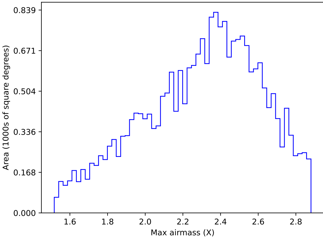
weather_cloudso8v3.4_10yrs All sky y band: Max airmass
