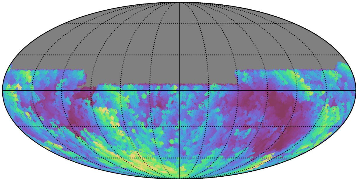
weather_cloudso8v3.4_10yrs All sky u band: Max airmass
