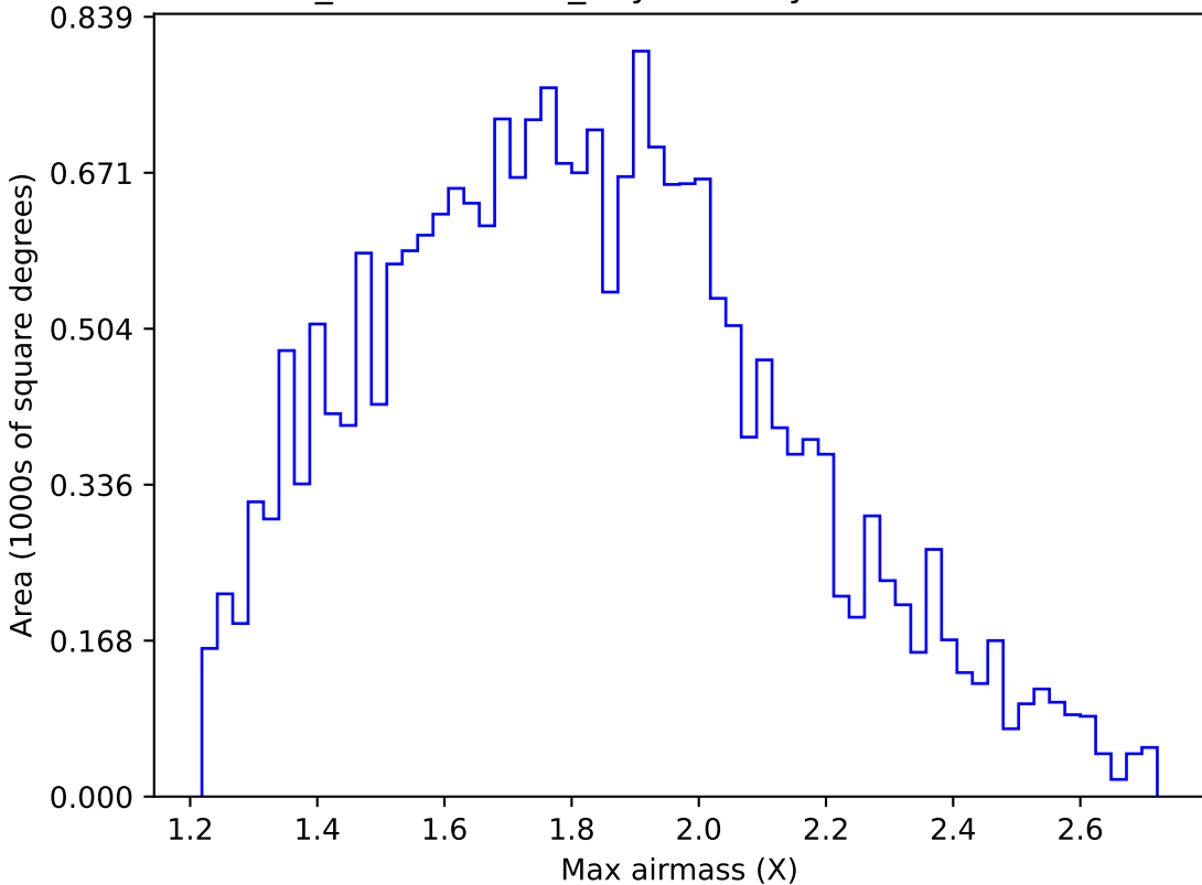
weather_cloudso8v3.4_10yrs All sky u band: Max airmass
