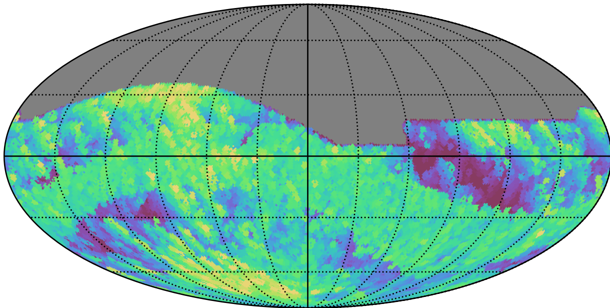
weather_cloudso8v3.4_10yrs All sky r band: Max airmass
