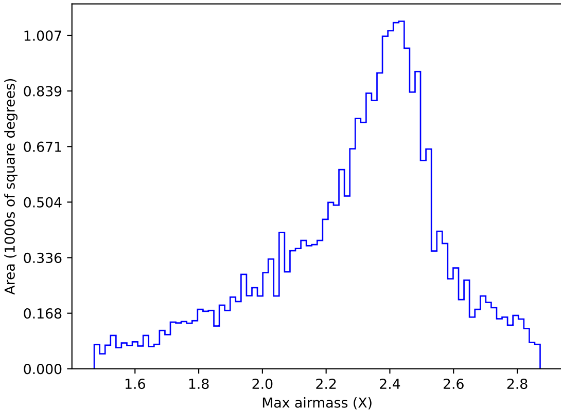
weather_cloudso8v3.4_10yrs All sky r band: Max airmass
