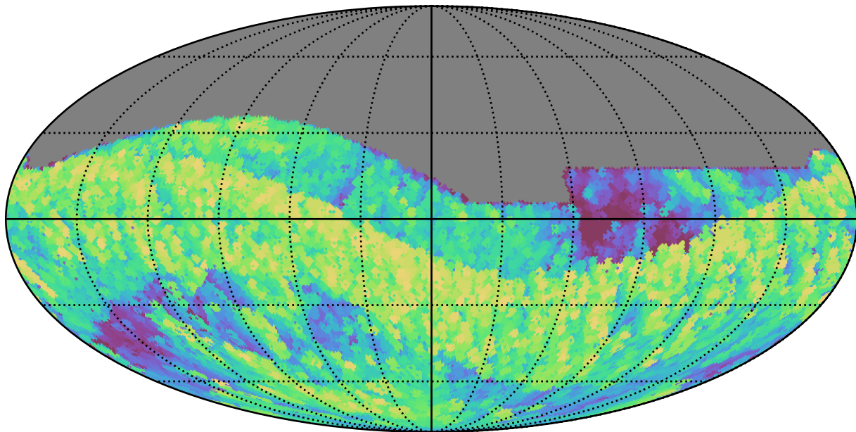
weather_cloudso8v3.4_10yrs All sky i band: Max airmass
