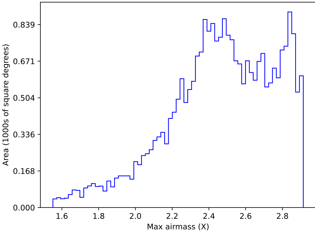
weather_cloudso8v3.4_10yrs All sky i band: Max airmass
