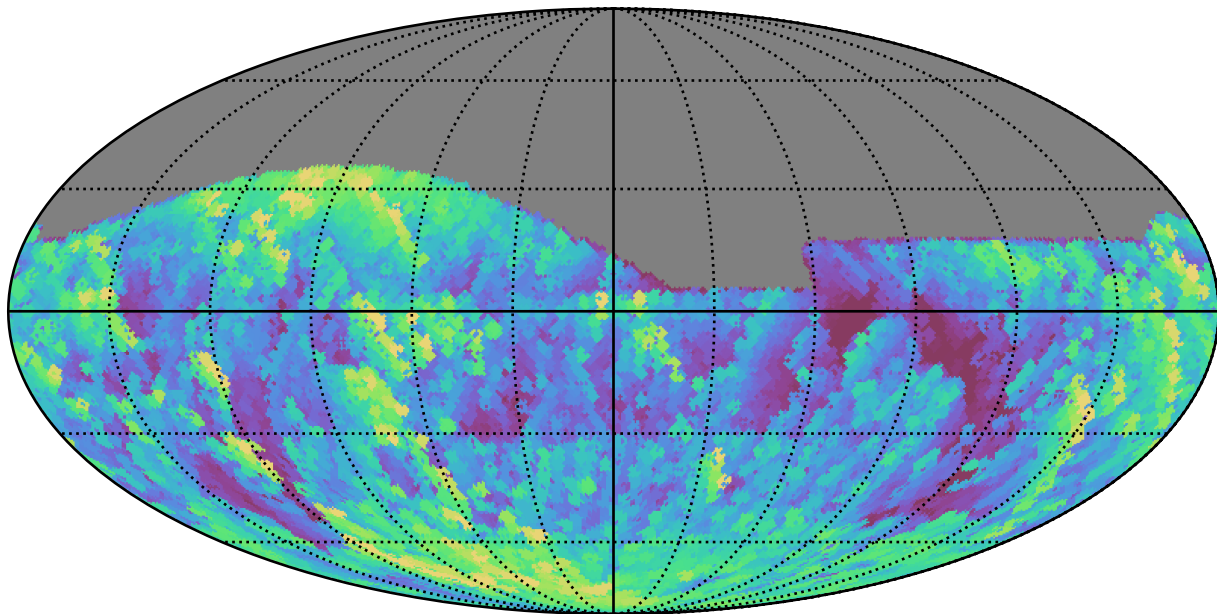
weather_cloudso8v3.4_10yrs All sky g band: Max airmass
