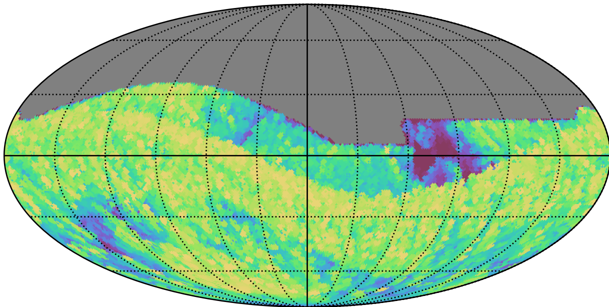
weather_cloudso8v3.4_10yrs All sky all bands: Max airmass
