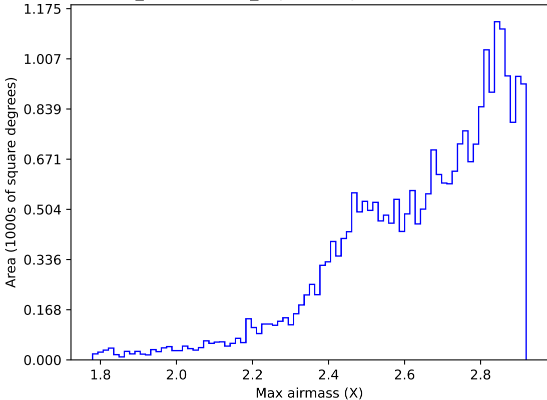
weather_cloudso8v3.4_10yrs All sky all bands: Max airmass
