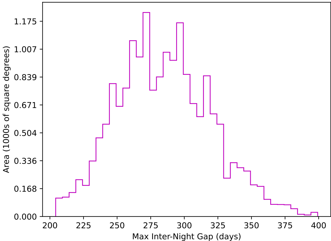
weather_cloudso8v3.4_10yrs WFD z band: Max Inter-Night Gap
