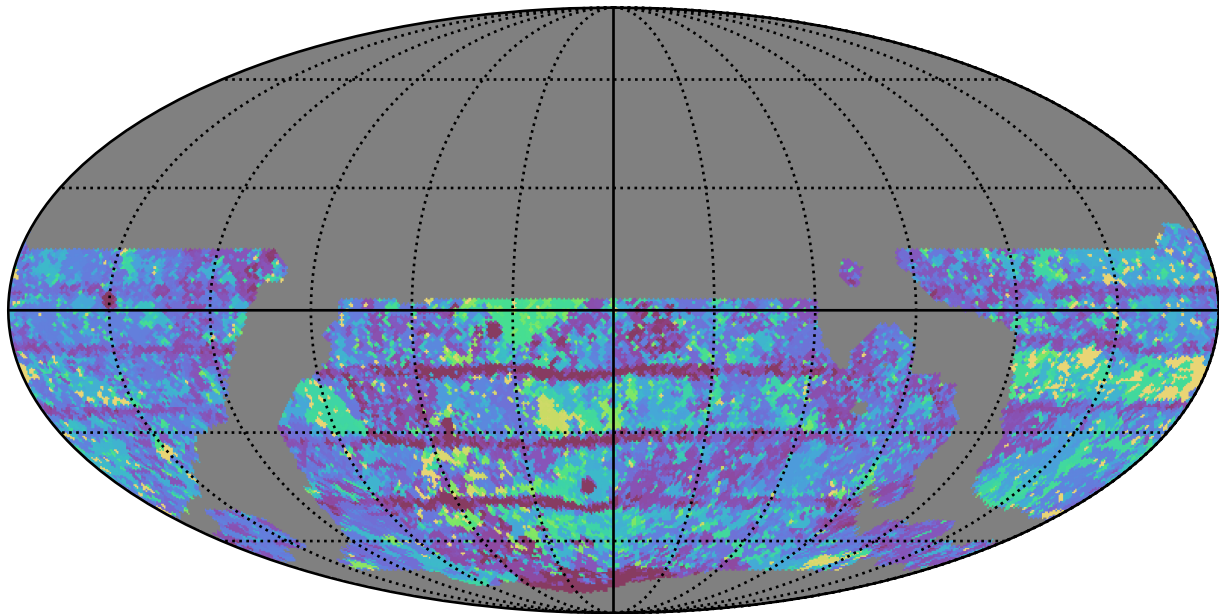
weather_cloudso8v3.4_10yrs WFD y band: Max Inter-Night Gap
