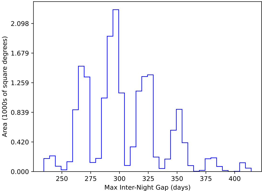
weather_cloudso8v3.4_10yrs WFD y band: Max Inter-Night Gap
