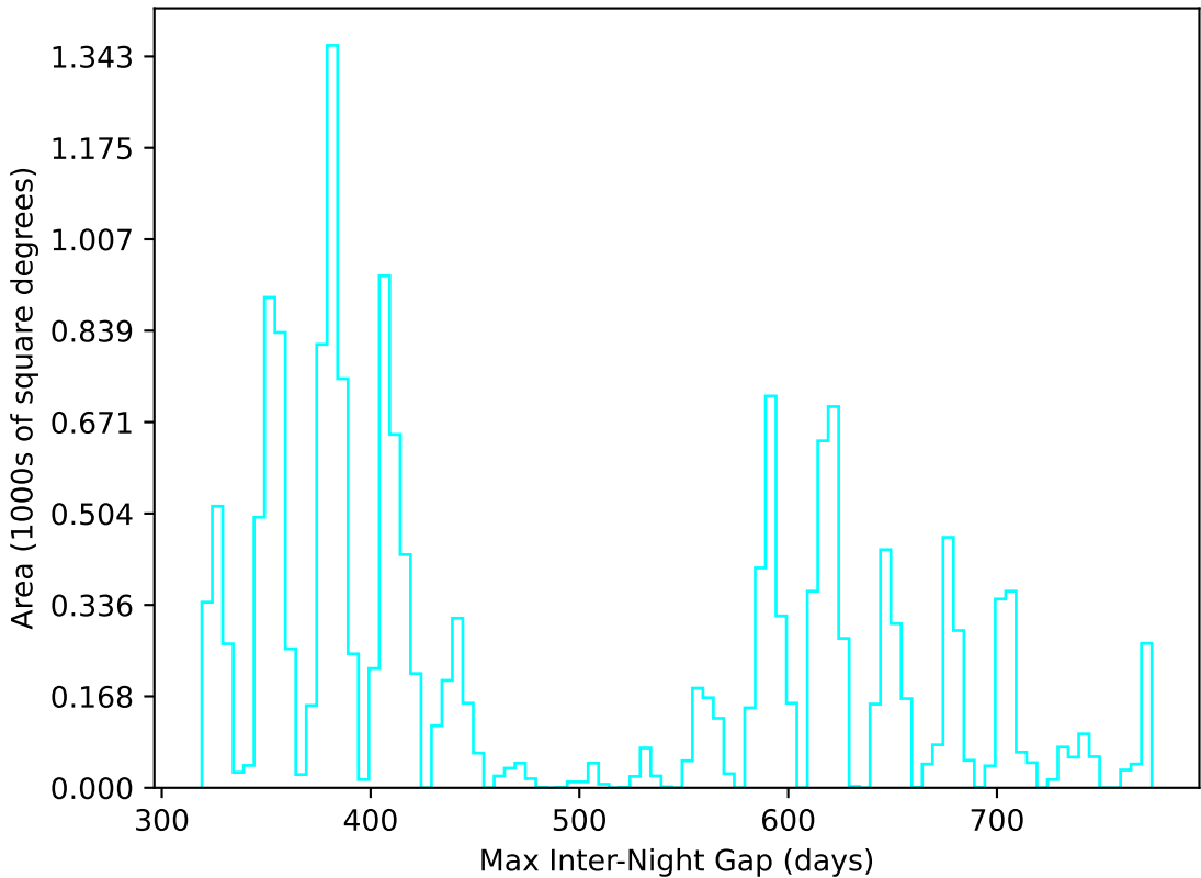
weather_cloudso8v3.4_10yrs WFD u band: Max Inter-Night Gap
