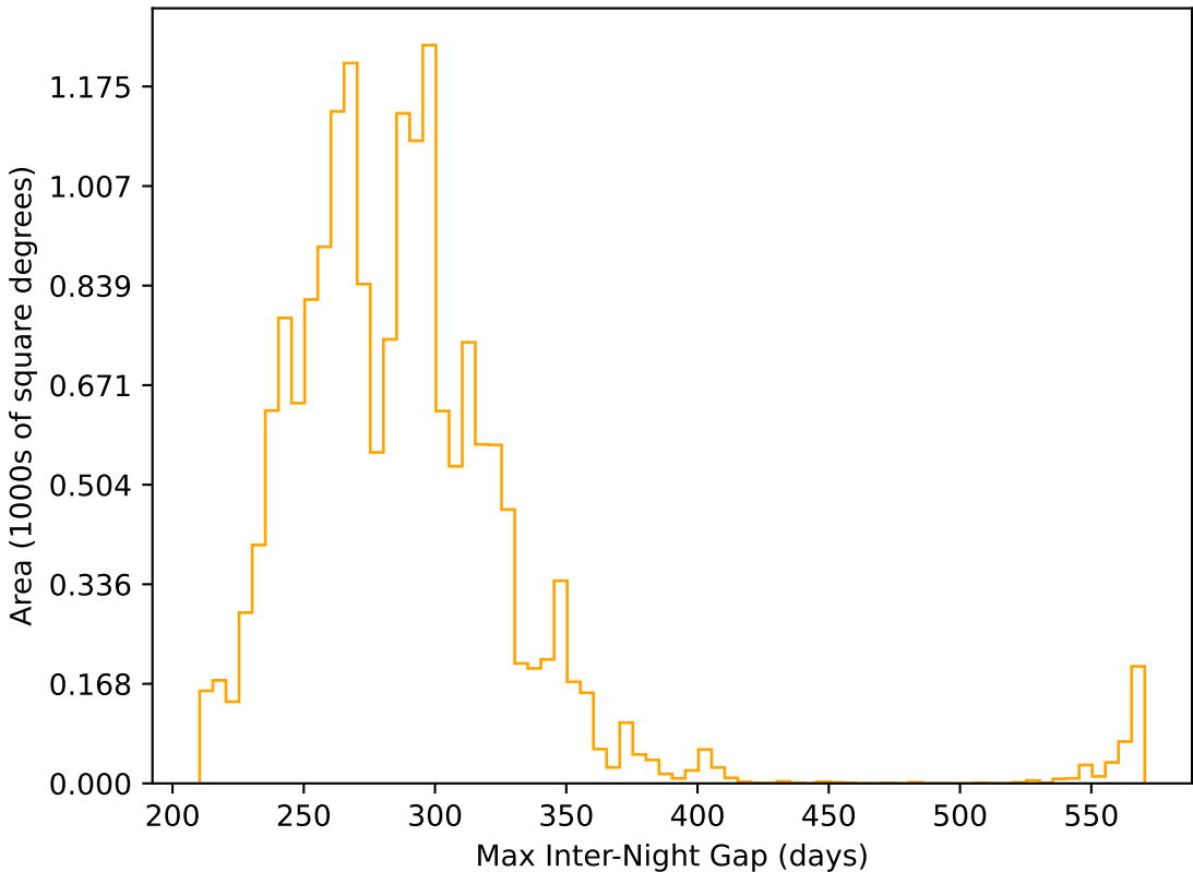
weather_cloudso8v3.4_10yrs WFD r band: Max Inter-Night Gap
