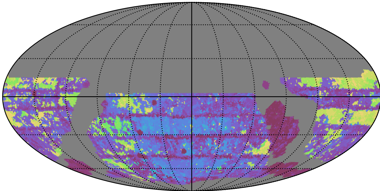
weather_cloudso8v3.4_10yrs WFD g band: Max Inter-Night Gap
