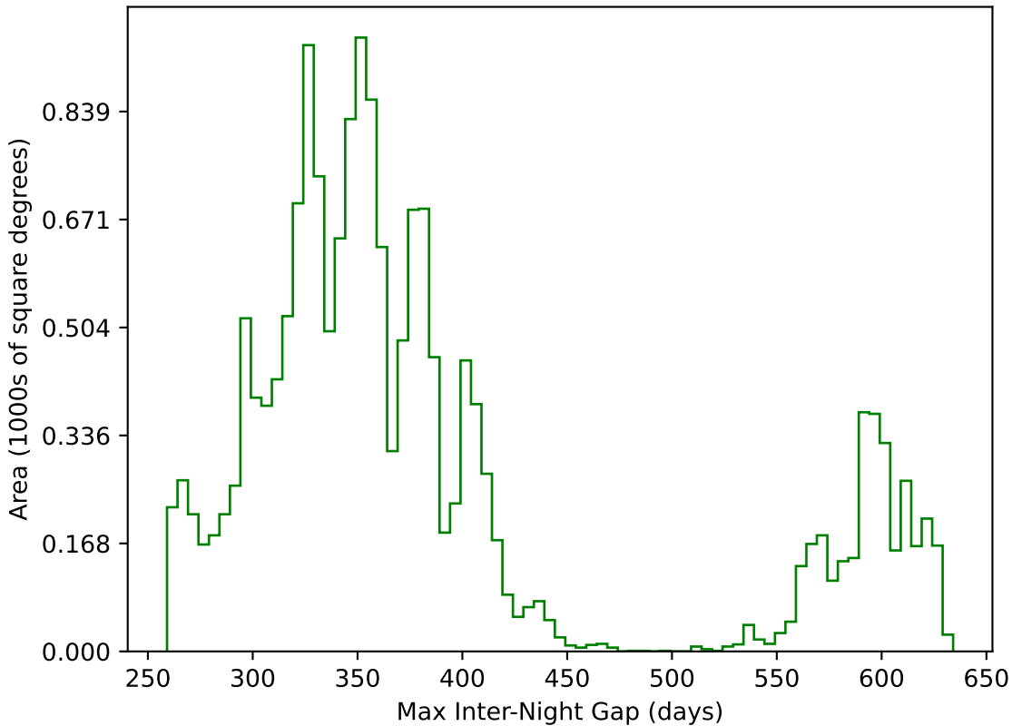
weather_cloudso8v3.4_10yrs WFD g band: Max Inter-Night Gap
