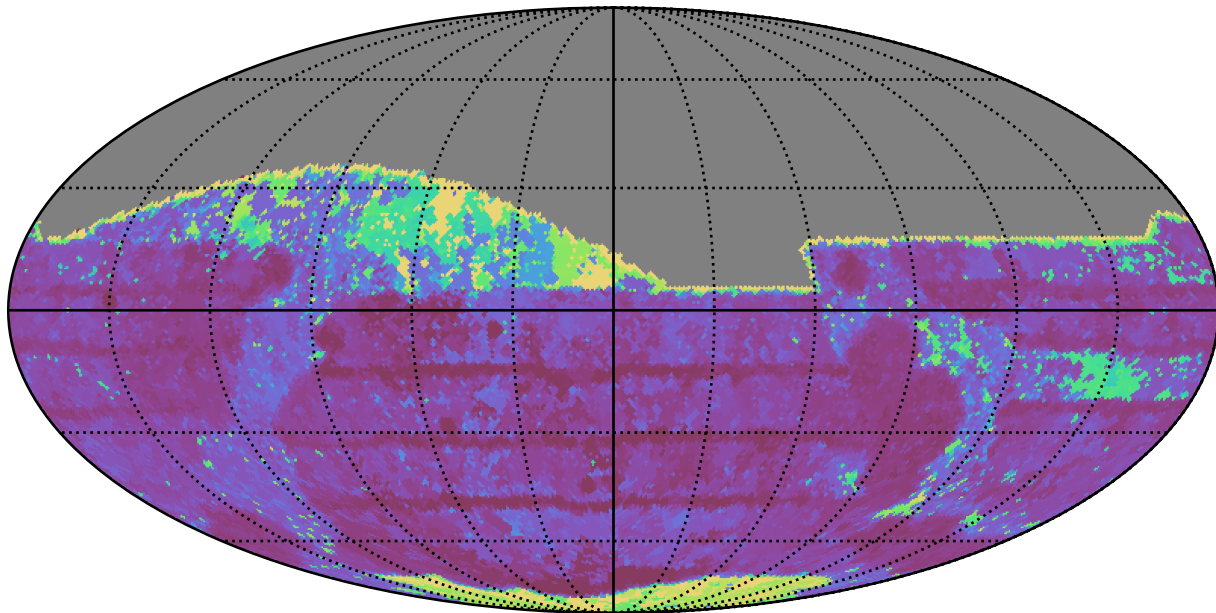
weather_cloudso8v3.4_10yrs All sky z band: Max Inter-Night Gap
