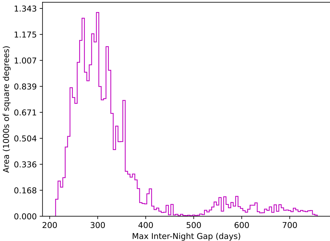
weather_cloudso8v3.4_10yrs All sky z band: Max Inter-Night Gap
