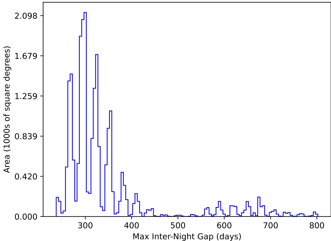
weather_cloudso8v3.4_10yrs All sky y band: Max Inter-Night Gap
