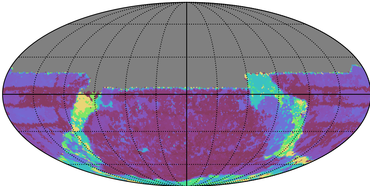
weather_cloudso8v3.4_10yrs All sky u band: Max Inter-Night Gap
