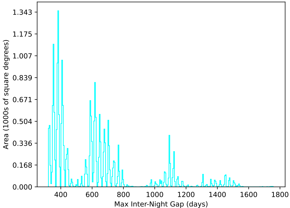
weather_cloudso8v3.4_10yrs All sky u band: Max Inter-Night Gap
