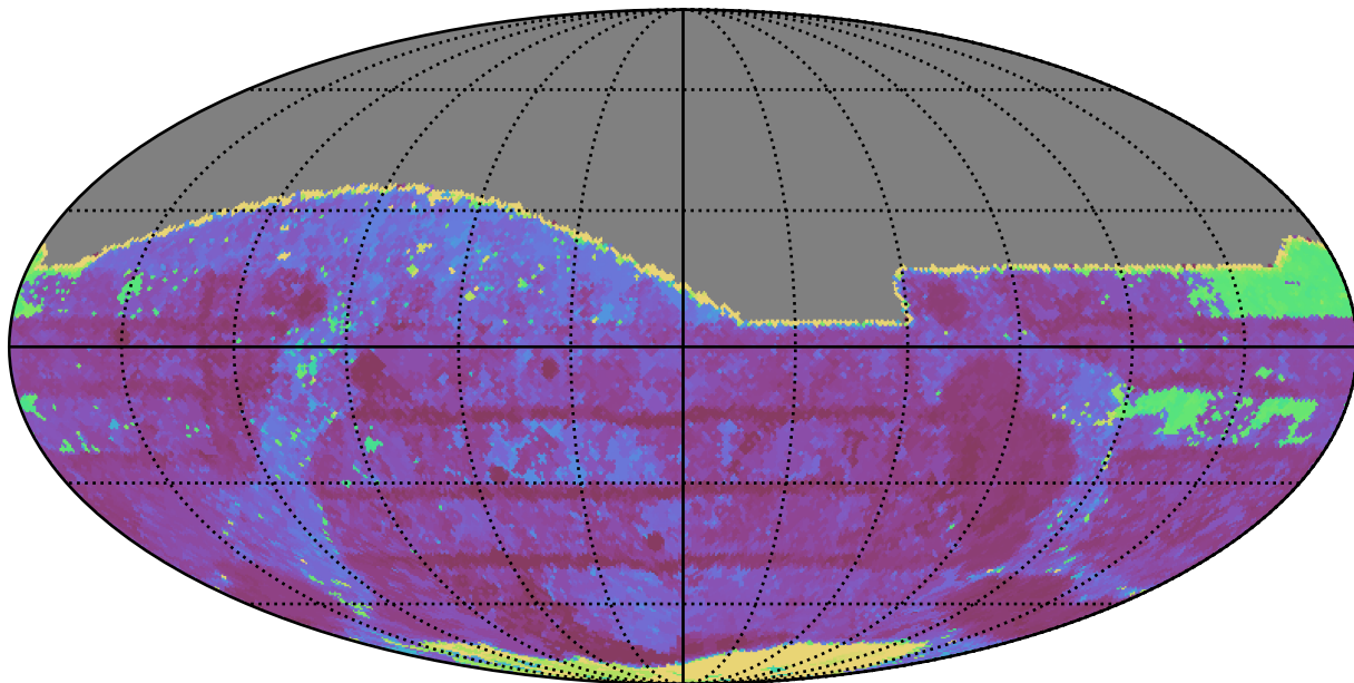
weather_cloudso8v3.4_10yrs All sky r band: Max Inter-Night Gap
