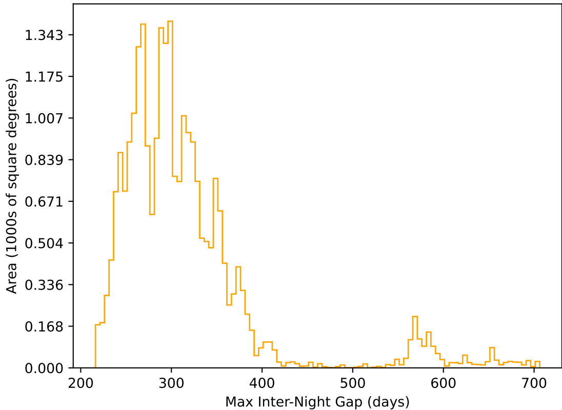
weather_cloudso8v3.4_10yrs All sky r band: Max Inter-Night Gap
