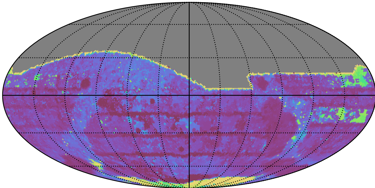
weather_cloudso8v3.4_10yrs All sky i band: Max Inter-Night Gap
