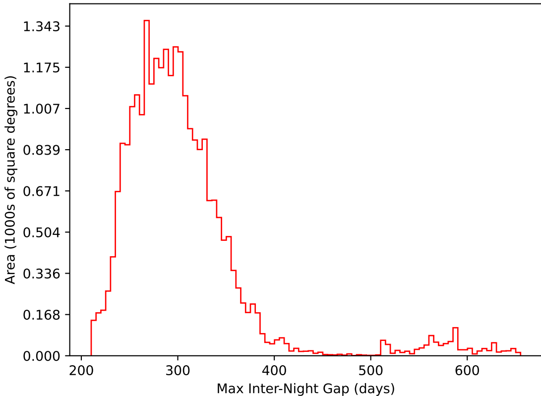
weather_cloudso8v3.4_10yrs All sky i band: Max Inter-Night Gap
