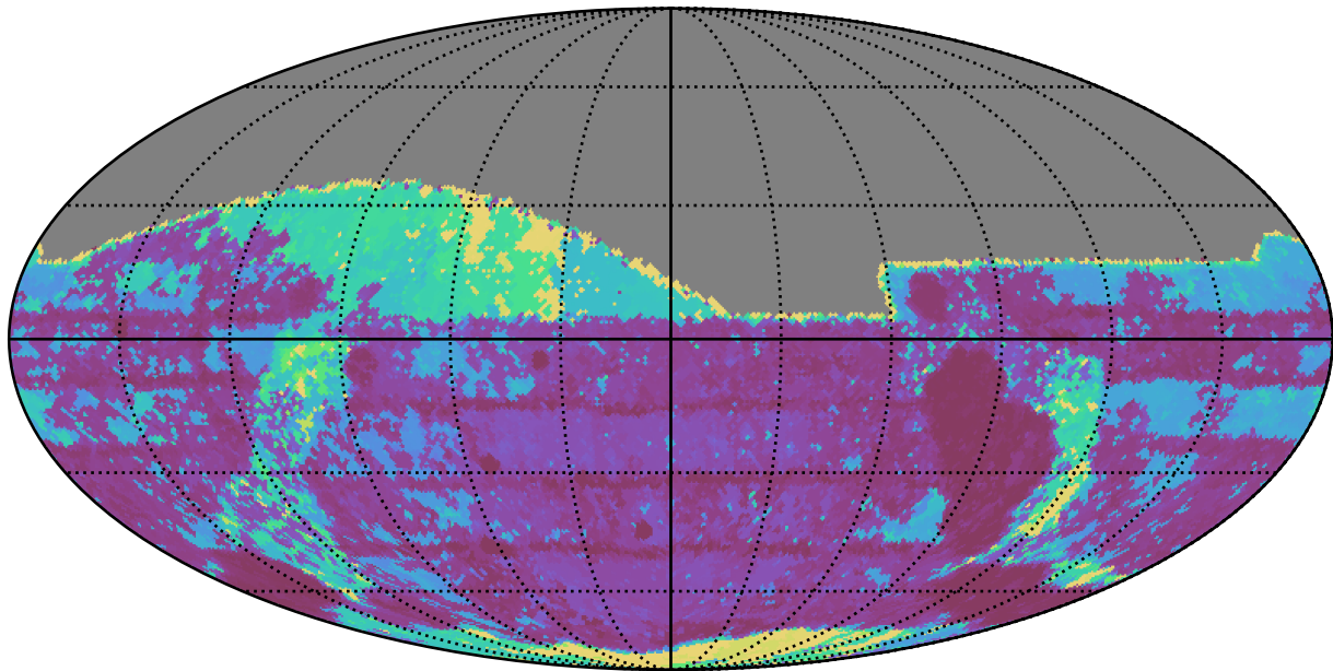
weather_cloudso8v3.4_10yrs All sky g band: Max Inter-Night Gap
