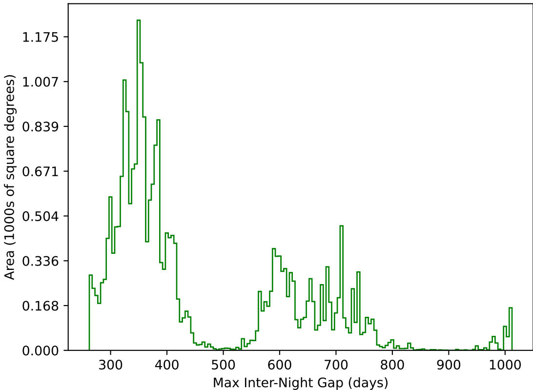
weather_cloudso8v3.4_10yrs All sky g band: Max Inter-Night Gap
